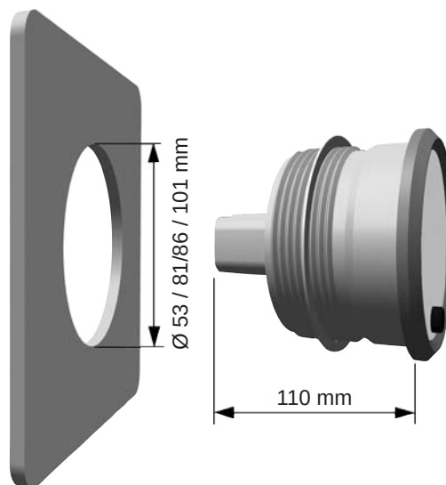
Fig. 6.3: Hole dimensions
