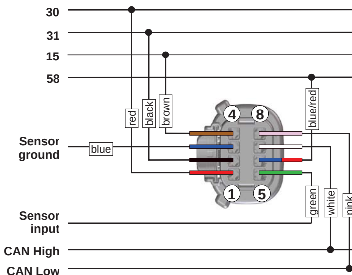
Fig. 3.2: Wiring diagram 8-pin connector
