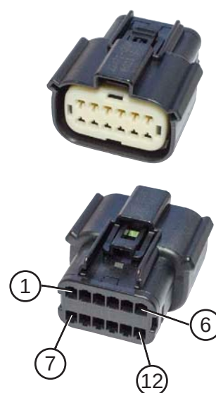
Fig. 6.5: MOLEX 12-pin connector
