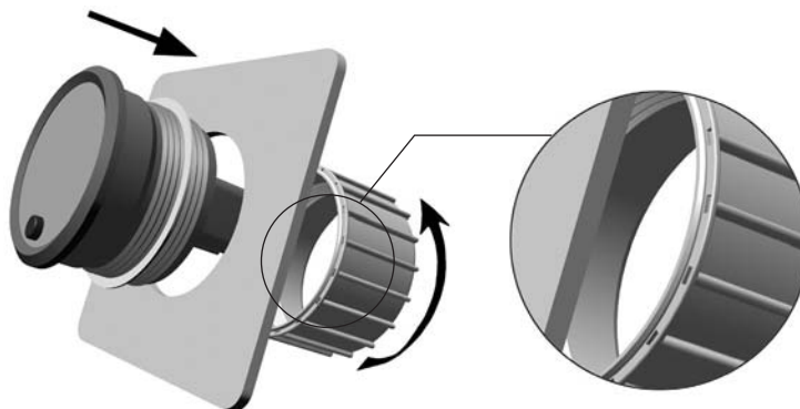
Fig. 6.6: Mount the gauge.
